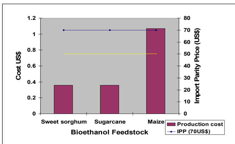
Figure 3 Comparison of production cost of ethanol from sweet sorghum, sugarcane and maize against import parity price of petrol (Source: CEEZ, ?)
