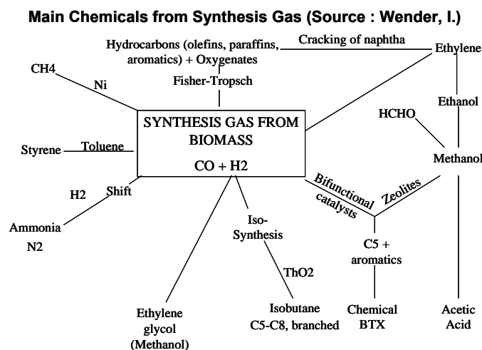
Figure 20: Main chemicals from synthesis gas
