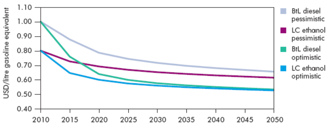
Figure 5: Cost projections for lignocellulosic ethanol and BTL diesel. (Source: IEA, 2008).
